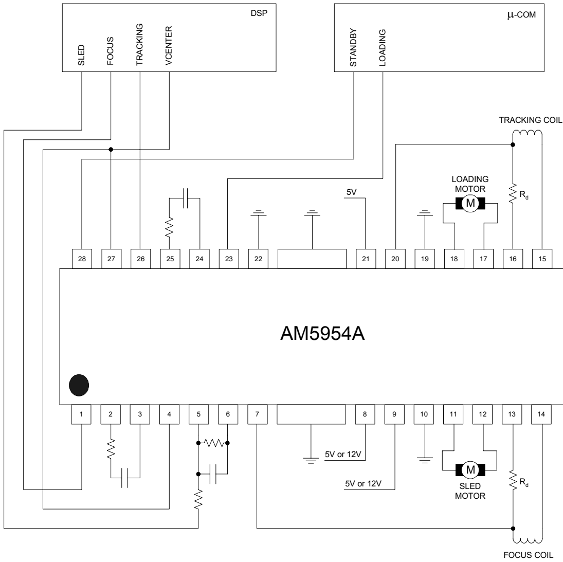
Figure 11. Typical Application of AM5954A in DVD Player
